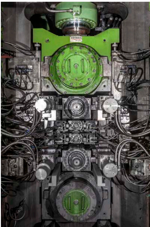
Rolling stand in six-high design with CVC ® plus.
