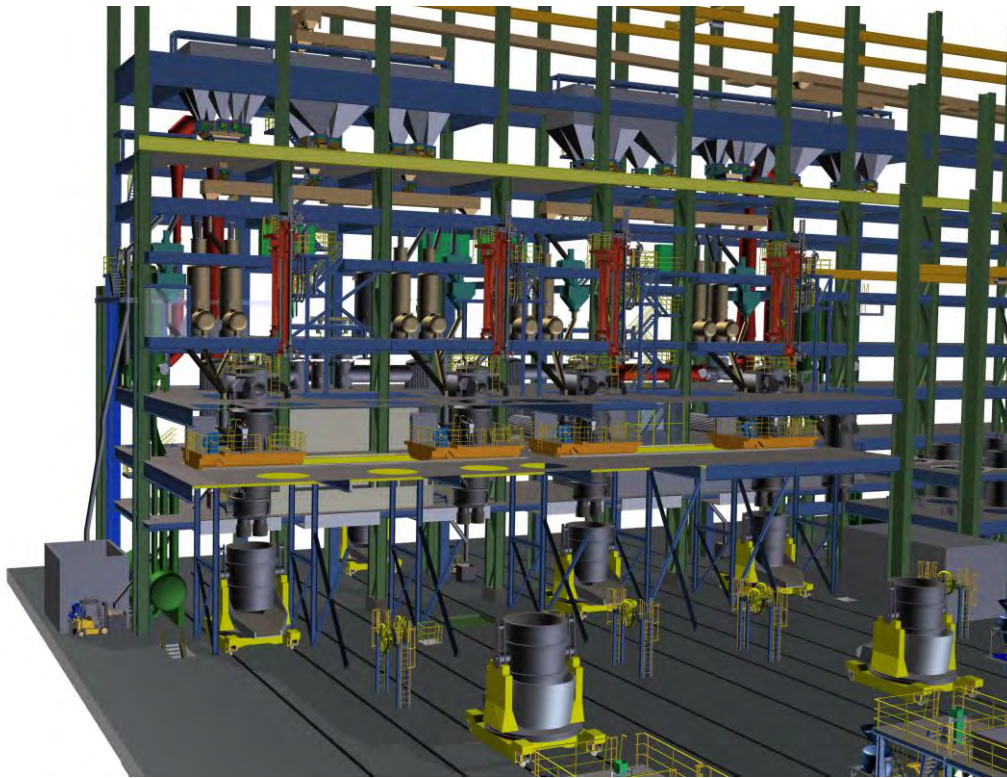
View of the 80-t Duplex RH-TOP plant.
